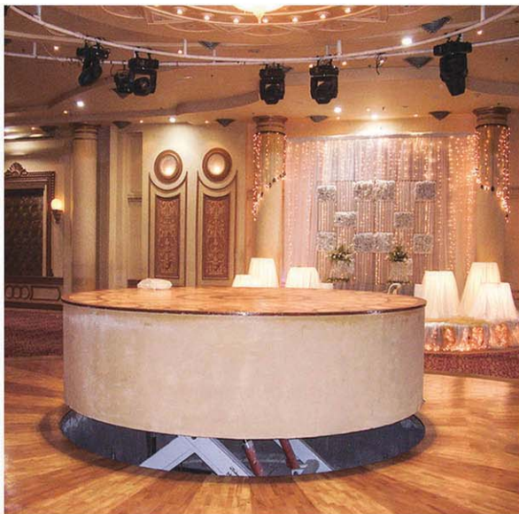
Stage Lift
